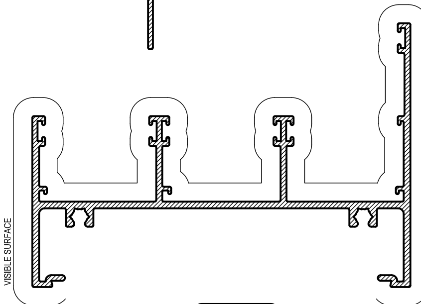
APT36s SLOTTED 101.6mm HIGH SILL
