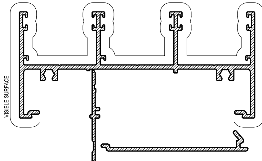
APT101 101.6mm REVEAL HEAD / JAMB
