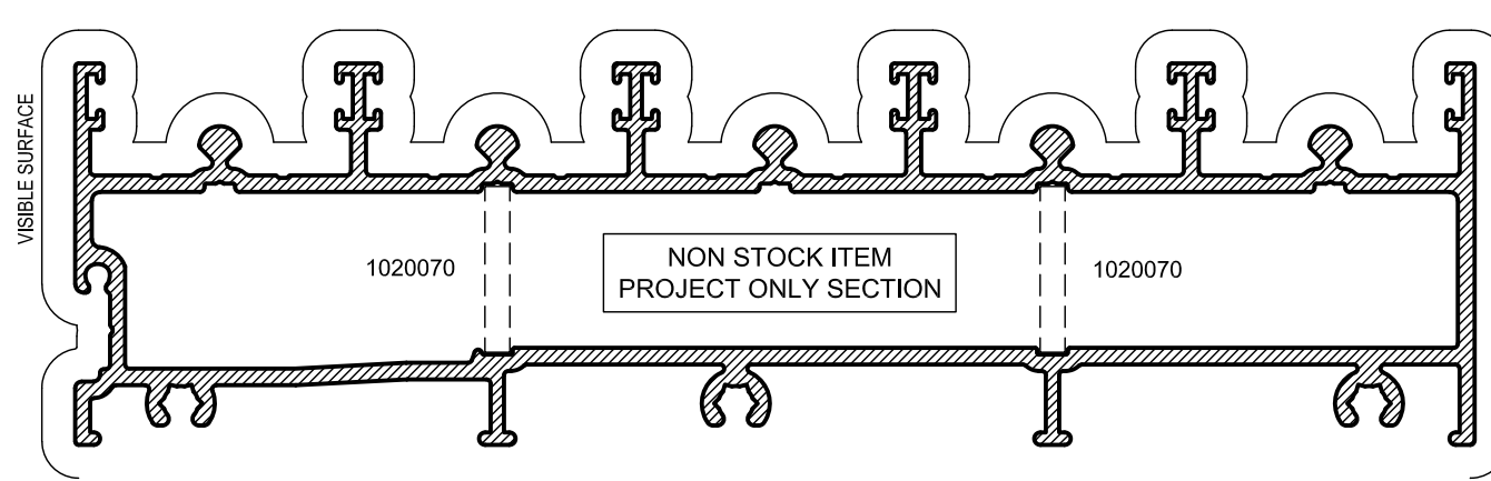
APT81S 5 TRACK HOLLOW SILL
