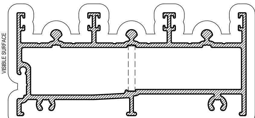
APT64S HOLLOW SILL (INCL TRACK)
