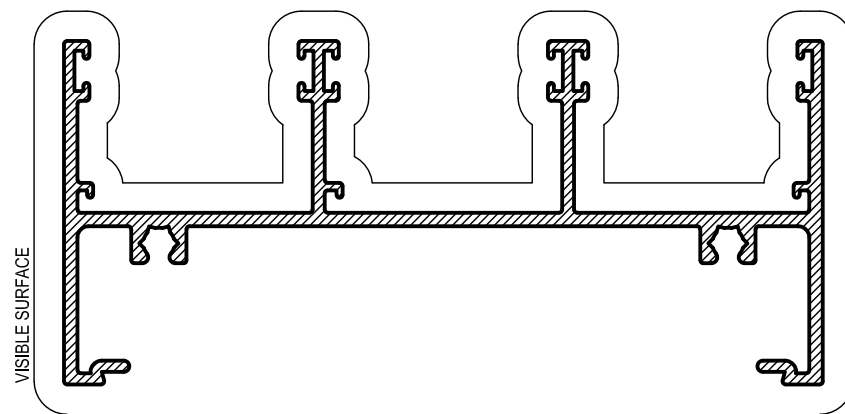
AS55 76mm FLAT INFILL
