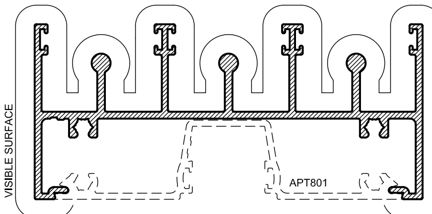
APT93S 101.6mm STANDARD SILL (SLOTTED)
