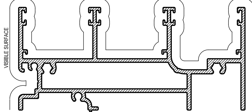
APT56S HOLLOW SILL
