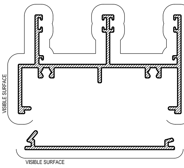
APT1 76mm HEAD / JAMB APT1s 76mm SLOTTED SILL
