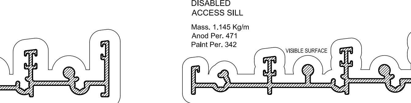
APT61 DISABLED ACCESS SILL
