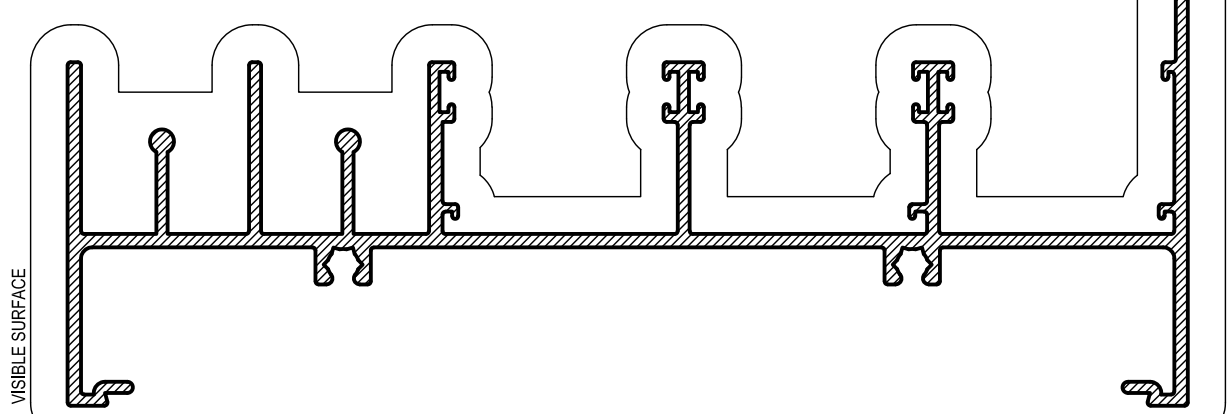
APT27 SILL SCREEN ADAPTOR
